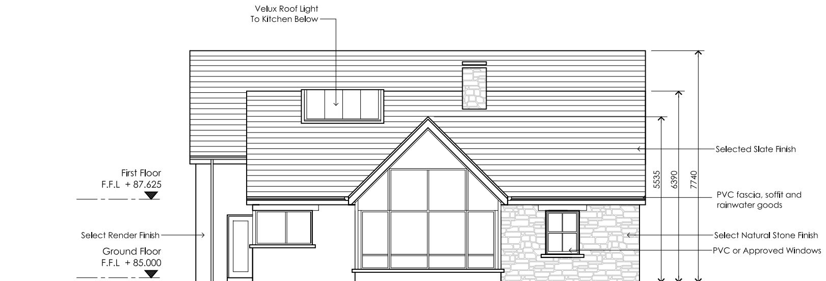
W ELEVATION - WEST
