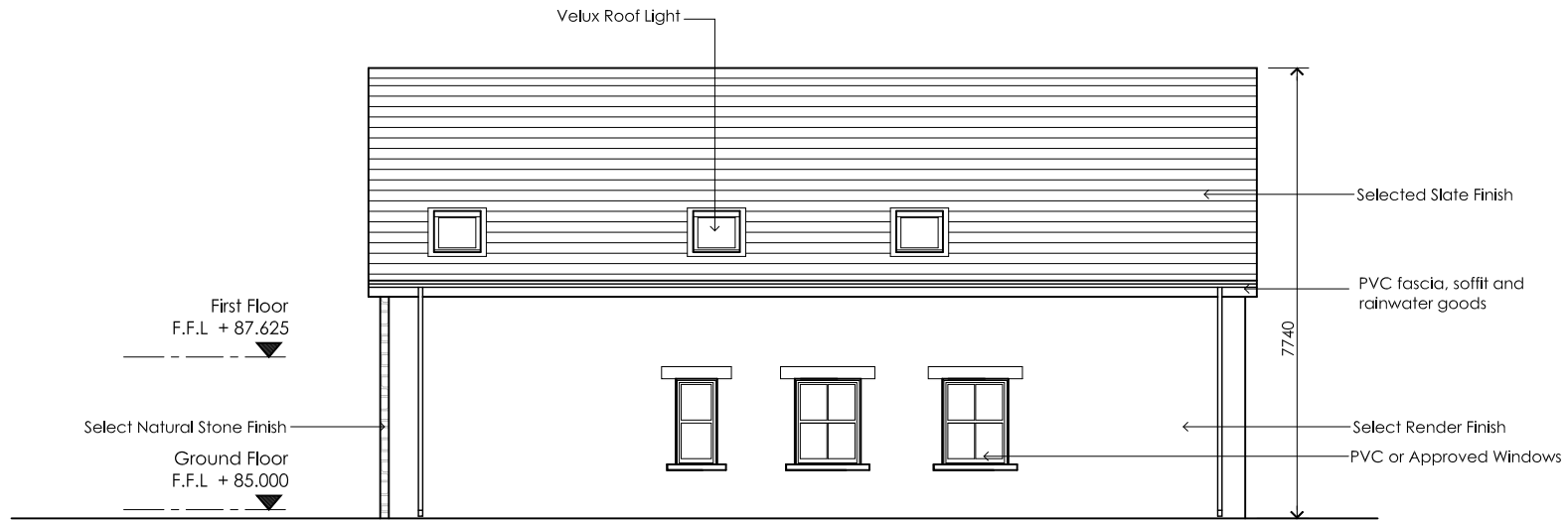
E ELEVATION - EAST
